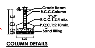
SCALE : 1: = 100
