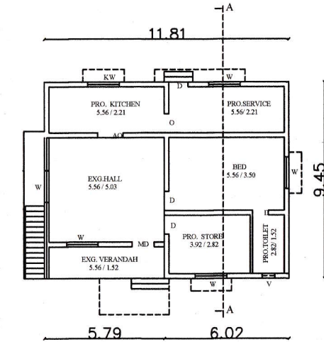
ECG & PRO. ADDL.GROUND FLOOR PLAN
