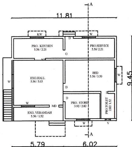
ECG & PRO. ADDL. GROUND FLOOR PLAN
