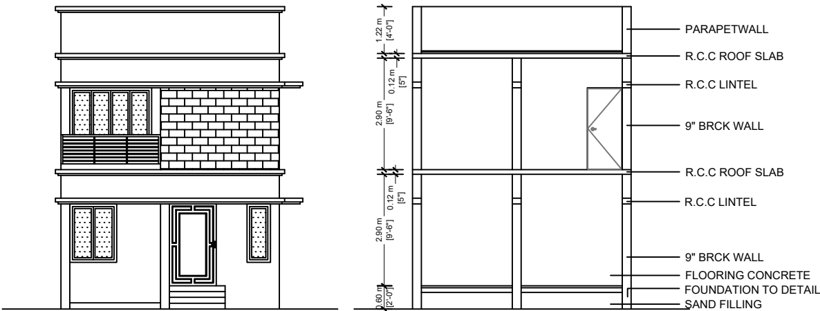
FRONT ELEVATION SECTION ON 'AA'
