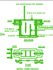
SEPTIC TANK DETAILS
