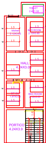
PROPOSED GROUND FLOOR PLAN
