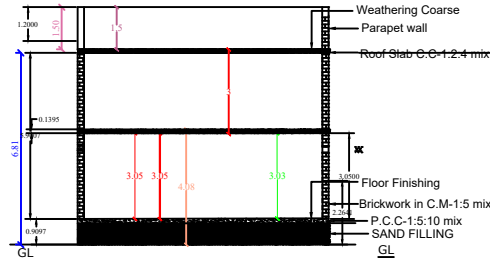
CROSS SECTION ON AB
