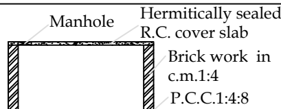
Section On 'Y-Y'
