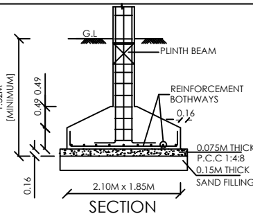
FOUNDATION DETAILS
