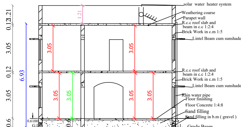
CROSS SECTION ON "A & A"
