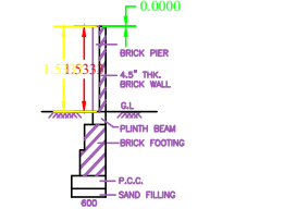
COMPOUND WALL
