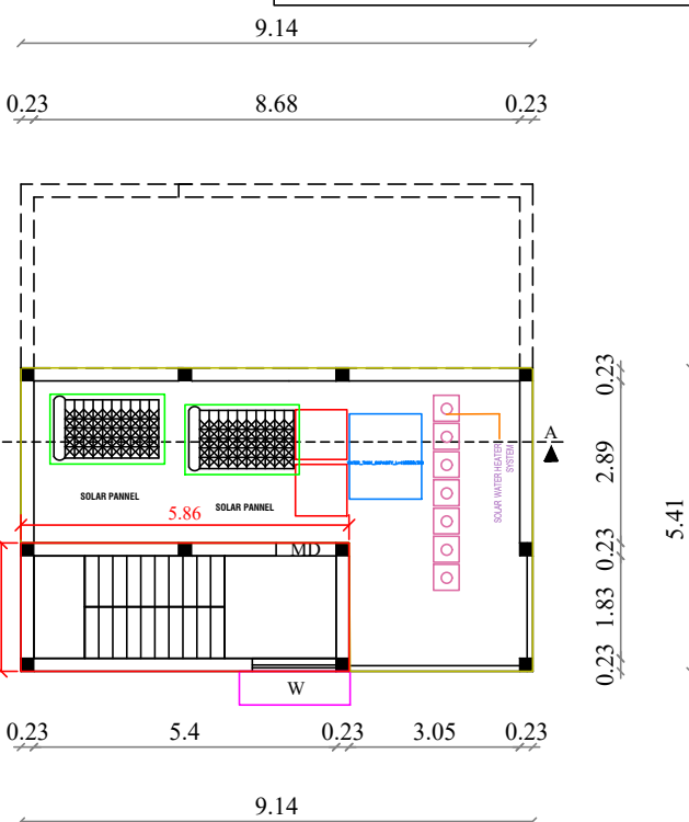
TERRACE -HEAD ROOM FLOOR
