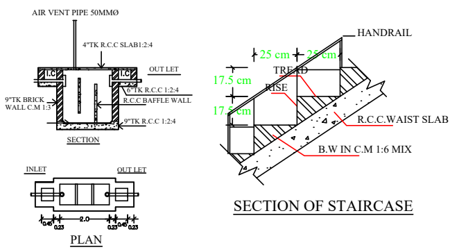
SEPTIC TANK DETAILS
