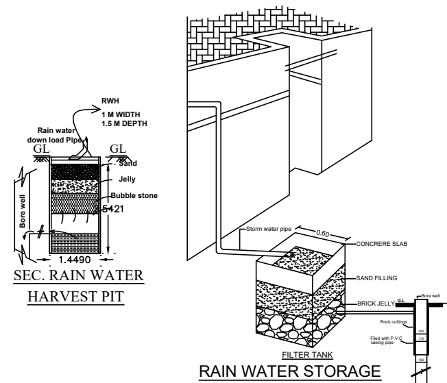
RAIN WATER STORAGE
