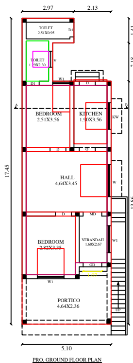
PRO. GROUND FLOOR PLAN
