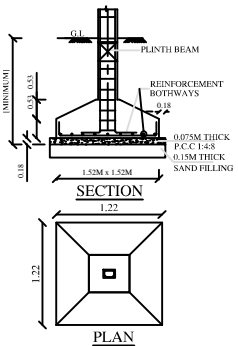
FOUNDATION DETAILS
