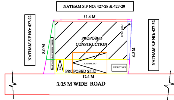
SITE PLAN
