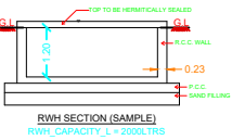
RW SECTION (SAMPLE) RW CAPACITY 1 = 2000 LTRS
