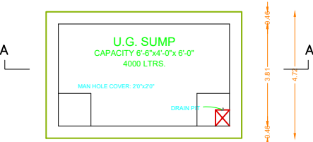
SUMP DETAIL SCALE 1"=4'0"
