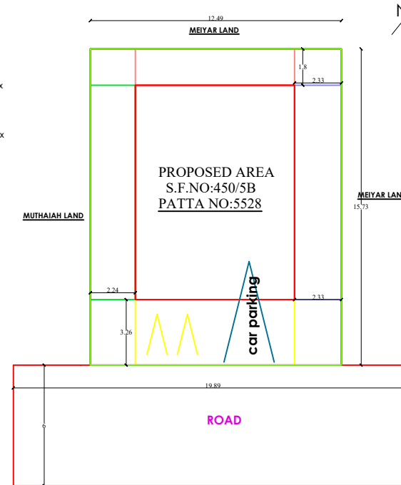
SITE PLAN-SCALE:100
