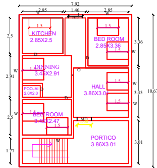
PROPOSED GROUND FLOOR PLAN
