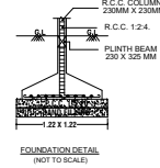
FOUNDATION DETAIL (NOT TO SCALE)
