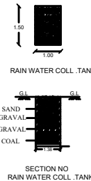
SECTION NO RAIN WATER COLL. TANK
