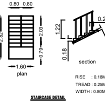
STAIRCASE DETAIL
