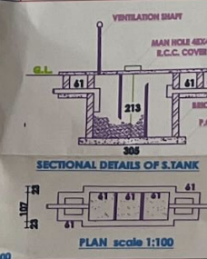
SECTIONAL DETAILS OF S.TANK
