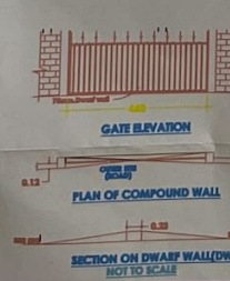
PLAN OF COMPOUND WALL
