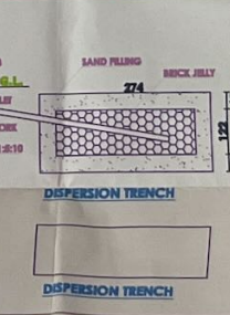
DISPERSION TRENCH
