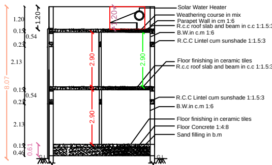
SECTION - "AB - CD "
