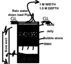
SEC. RAIN WATER HARVEST PIT
