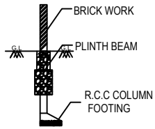
SECTION
