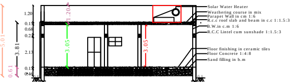
SECTION - "AB "
