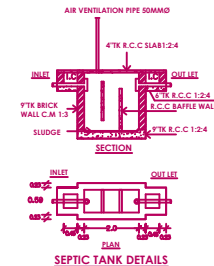
SEPTIC TANK DETAILS
