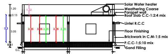
SECTION"AB"
