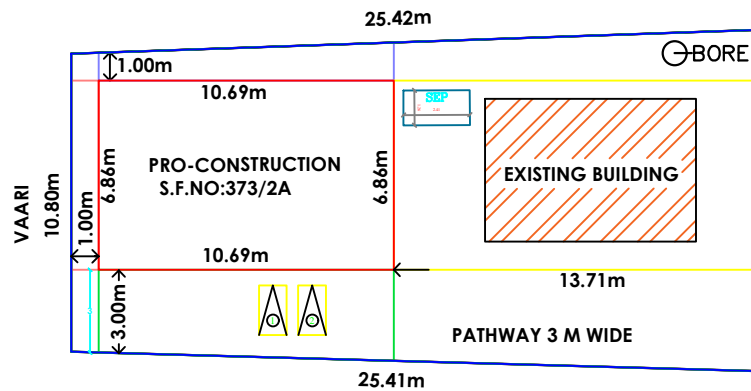
KULATHI KOOLAIYAR PUNJAI SITE PLAN-SCALE1:100
