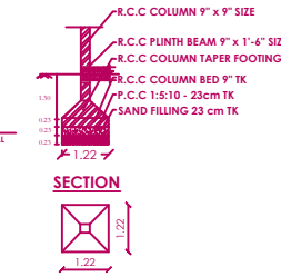
COLUMN DETAILS PLAN
