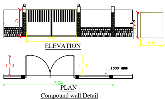
Compound wall Detail
