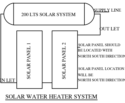
SOLAR WATER HEATER SYSTEM
