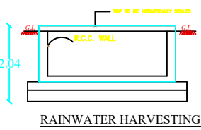
RAINWATER HARVESTING
