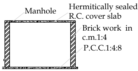
Section On 'Y-Y'
