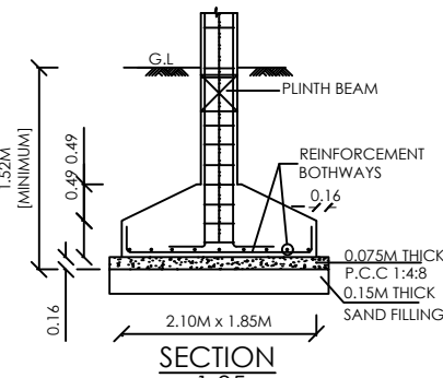
SECTION 1.85
