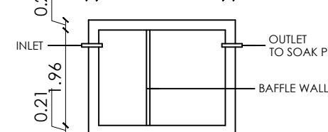
PLAN SEPTIC TANK
