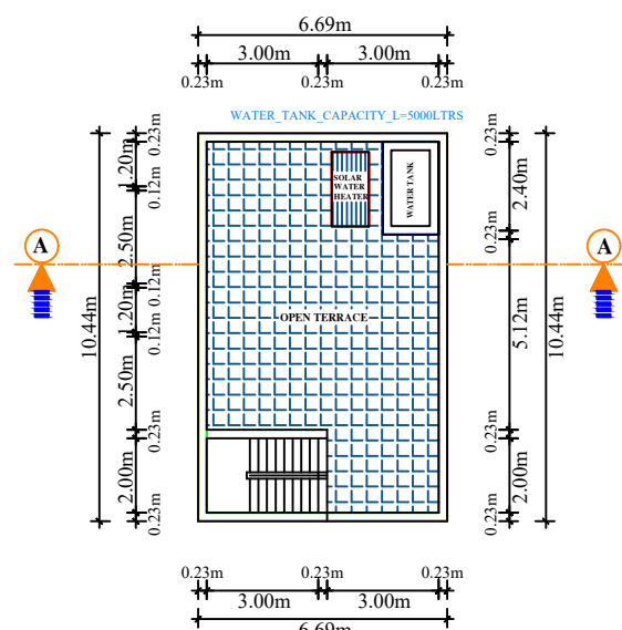
TERRACE PLAN
