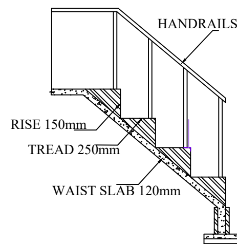
STAIRCASE DETAILS
