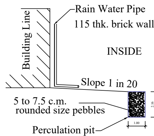
RAIN WATER HARVESTING PERCUSSION PIT RW_H_CAPACITY_L=2000LTRS
