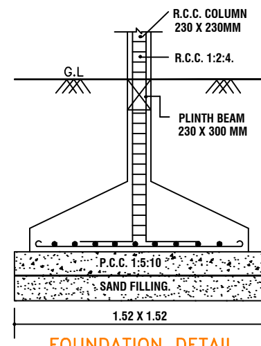
FOUNDATION DETAIL
