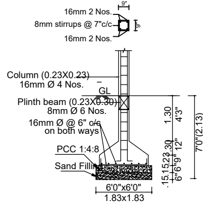
FOUNDATION DETAIL
