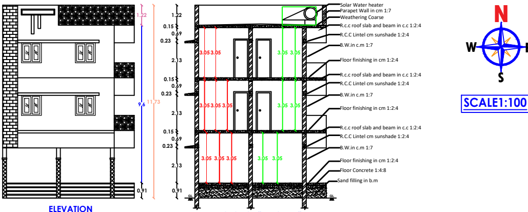
SECTION"AB,CD,EF"
