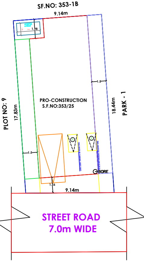
SITE PLAN-SCALE:1:100
