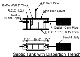
Septic Tank with Dispersal Trench
