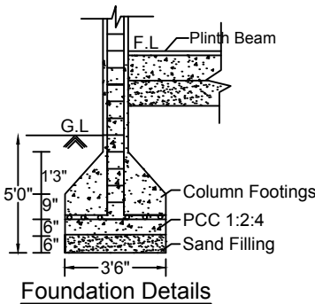
Foundation Details
