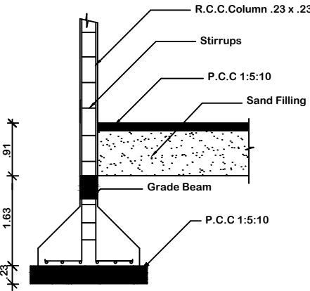
COLUMN DETAIL
