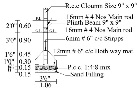
COLUMN DETIAL
