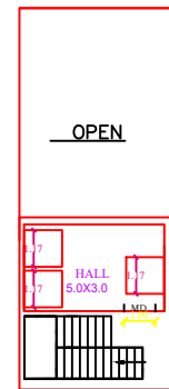
EXISTING FIRST FLOOR PLAN
