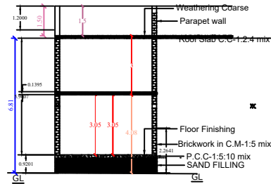
CROSS SECTION ON AB
