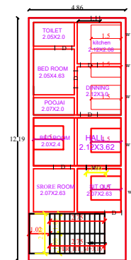
EXISTING GROUND FLOOR PLAN
