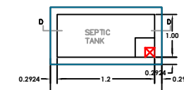
PLAN OF SEPTIC TANK SCALE 1"=2'-0"
