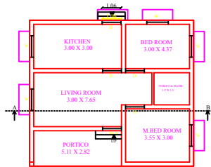
EXISTING GROUND FLOOR PLAN
