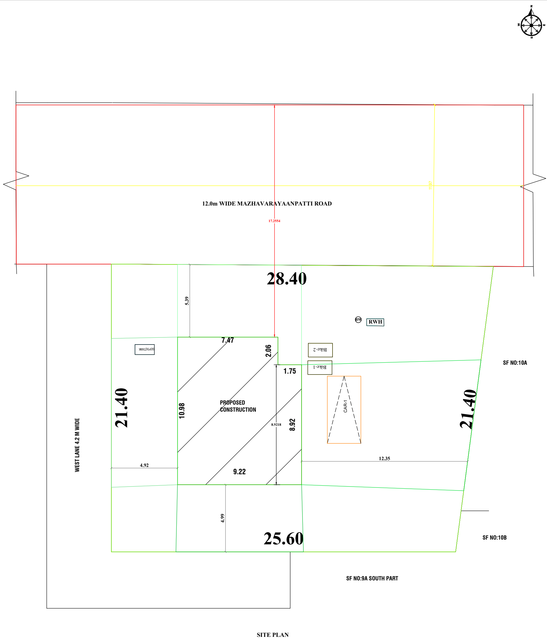
SITE PLAN
