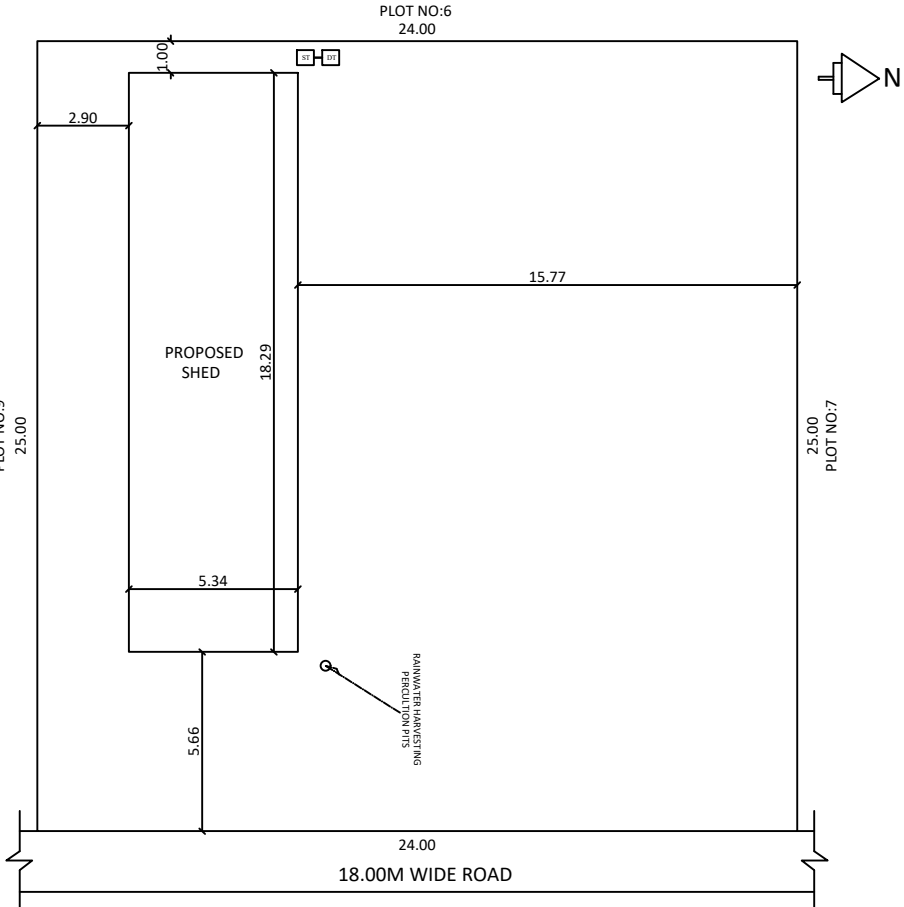
SITE PLAN
