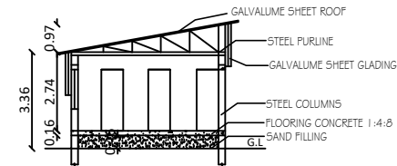
SECTION ON GG
