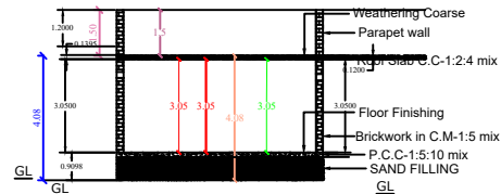
CROSS SECTION ON AB
