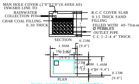
RWH_CAPACITY_L=5000LTRS
