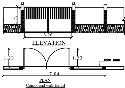
Compound wall Detail
