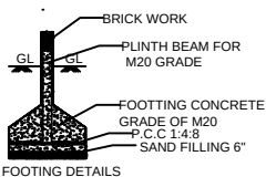
FOOTING DETAILS
