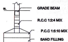
COLUMN DETAILS
