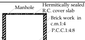
Section On 'Y-Y'
