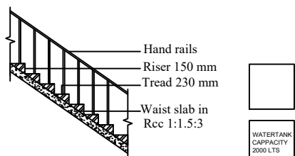
DETAILS OF STAIR CASE
