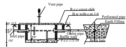
SECTION OF S.P.T &amp; D.T
