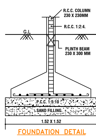
FOUNDATION DETAIL
