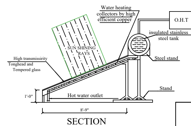
SECTION SOLAR WATER HEATER
