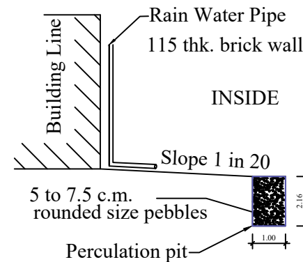
RAIN WATER HARVESTING PERCUSSION PIT RW_H_CAPACITY_L=2000LTRS
