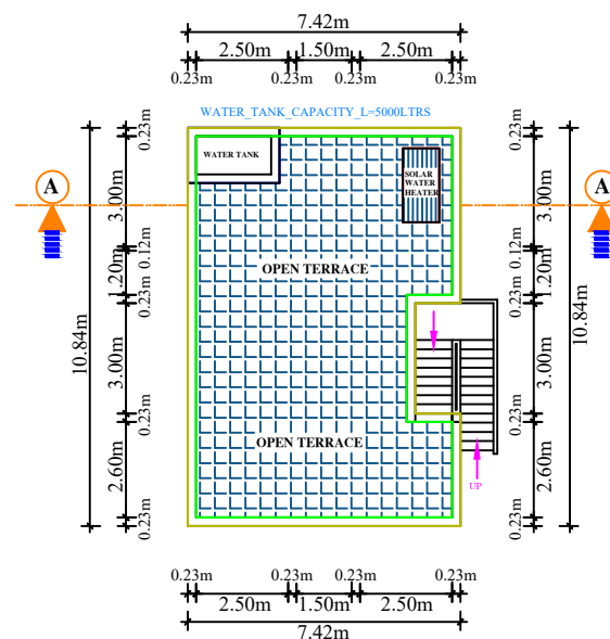
TERRACE PLAN
