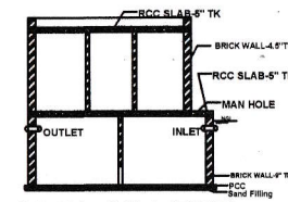
TOILET & SEPTIC TANK SECTION
