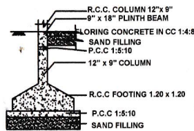
COLUMN FOOTING DETAILS
