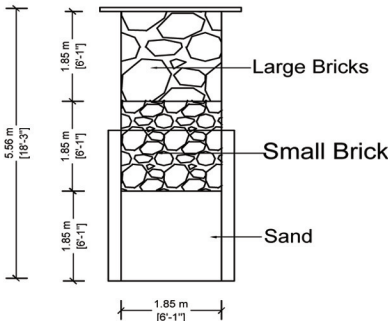
SECTION OF RAIN WATER COLLECTION PITS (NTS)
