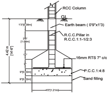
FOUNDATION DETAILS
