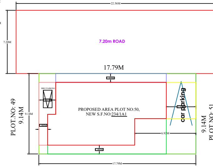
17.79M SF.NO: 234/1B SITE PLAN SCALE 1:100
