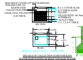
SECTION
