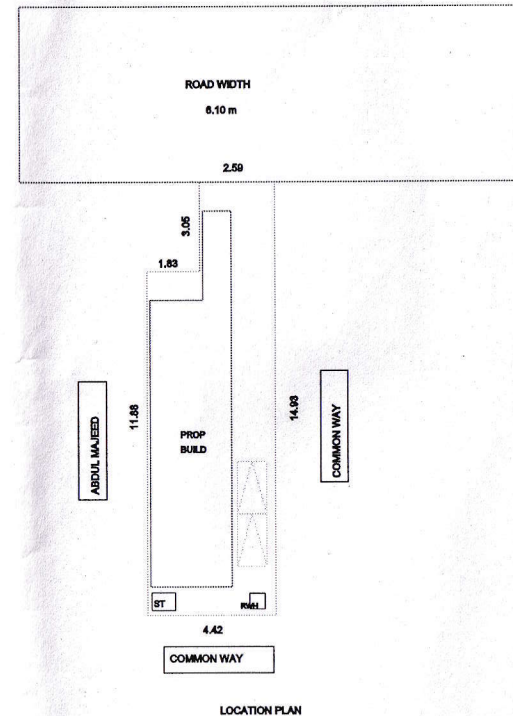
LOCATION PLAN
