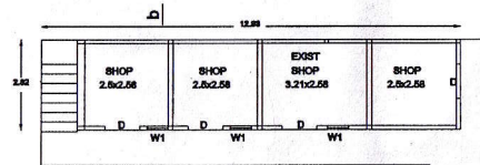
PROPOSED FIRST FLOOR
