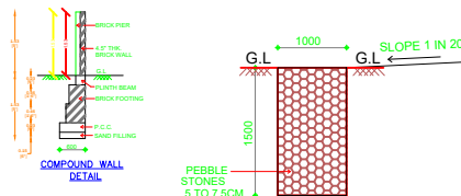
SECTION OF PEBBLE TRENCH SCALE : 1: = 100
