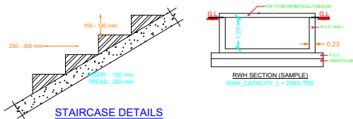
STAIRCASE DETAILS NOT TO SCALE
