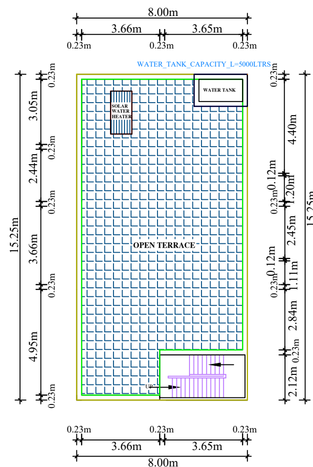
TERRACE PLAN
