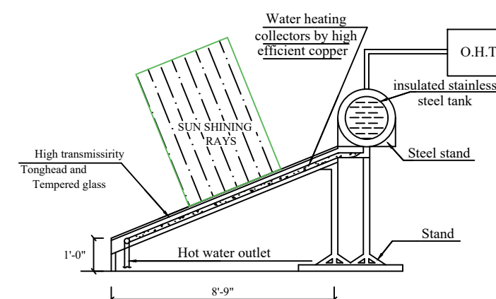
SECTION SOLAR WATER HEATER
