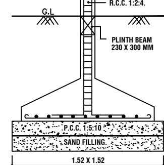
FOUNDATION DETAIL
