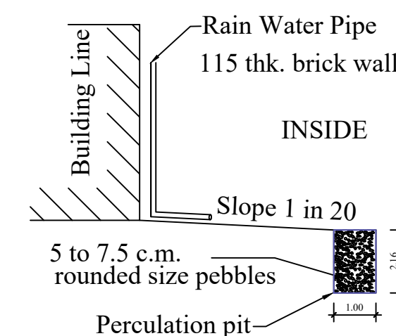
RAIN WATER HARVESTING PERCOLATION PIT RWH_CAPACITY_L=2000LTRS
