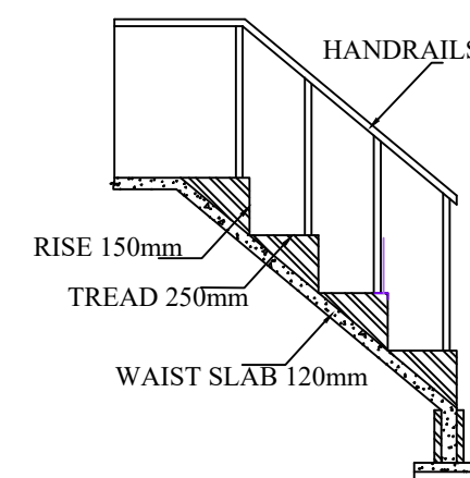
STAIRCASE DETAILS
