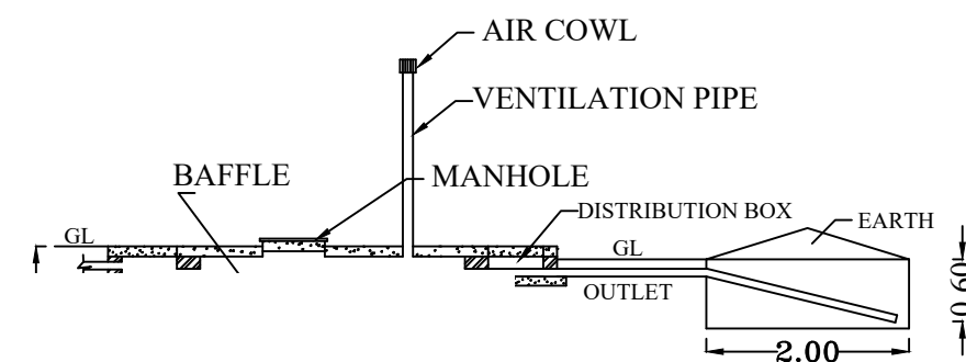
SECTION
