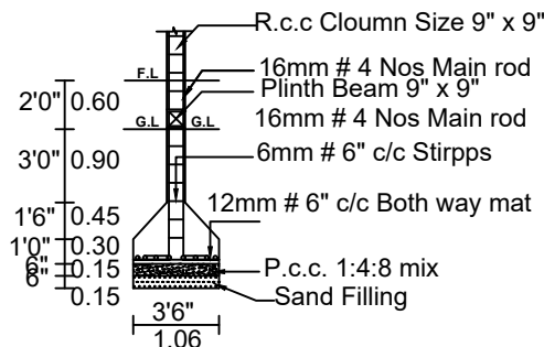
COLUMN DETIAL
