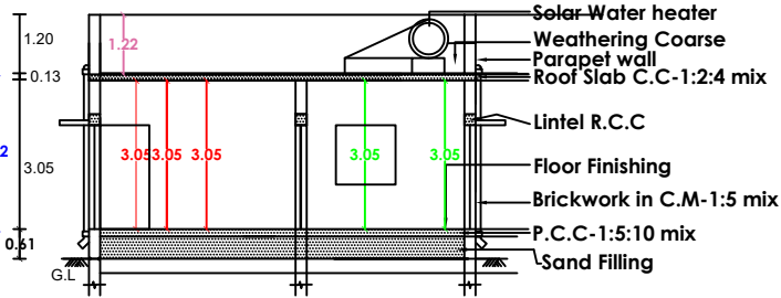
SECTION"AB"
