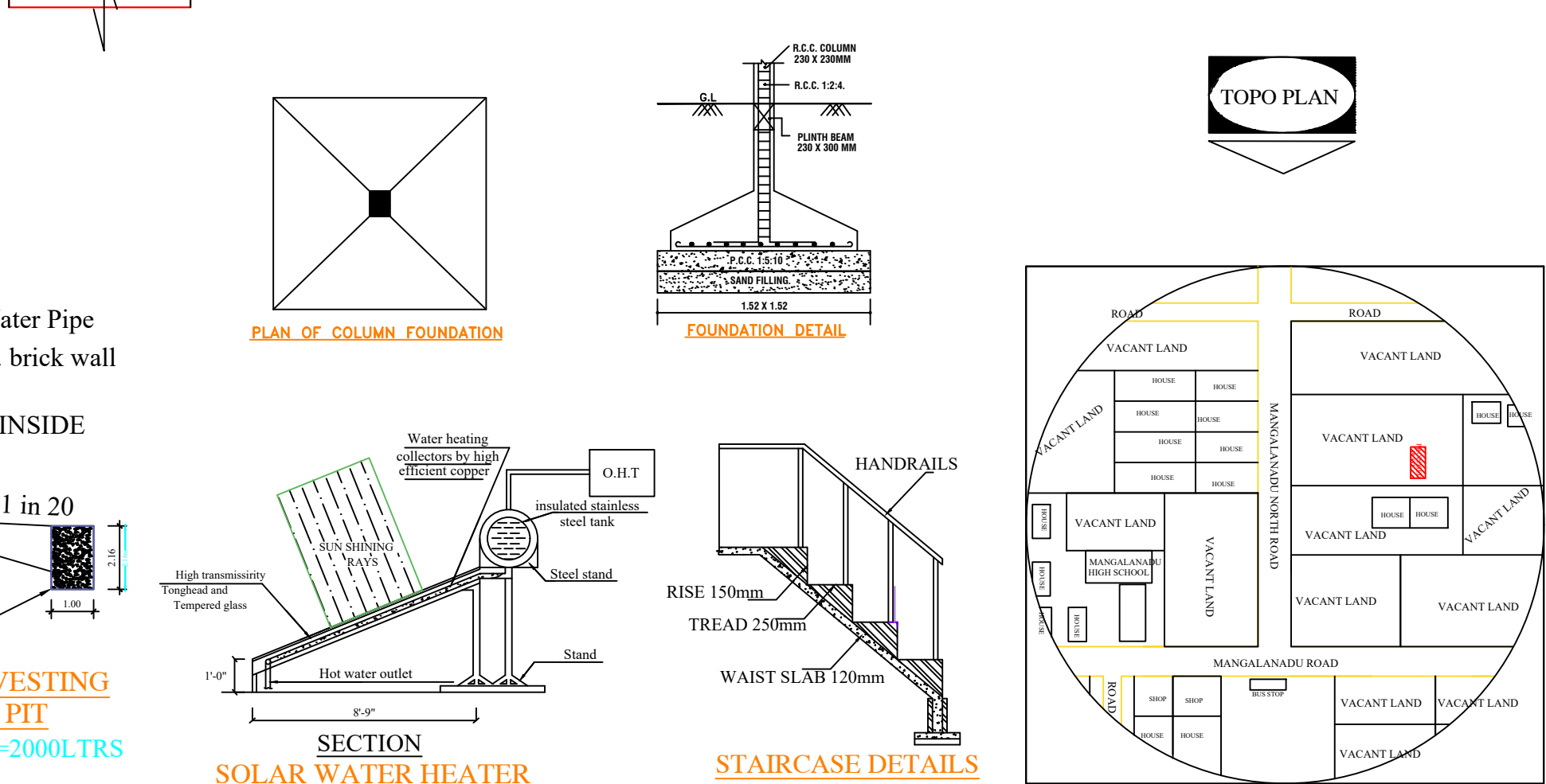
FOUNDATION DETAIL PLAN OF COLUMN FOUNDATION SOLAR WATER HEATER STAIRCASE DETAILS
