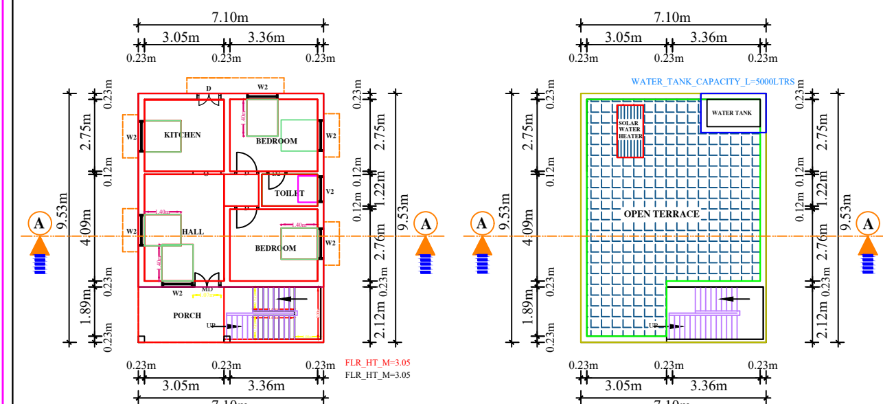
GROUND FLOOR PLAN TERRACE FLOOR PLAN
