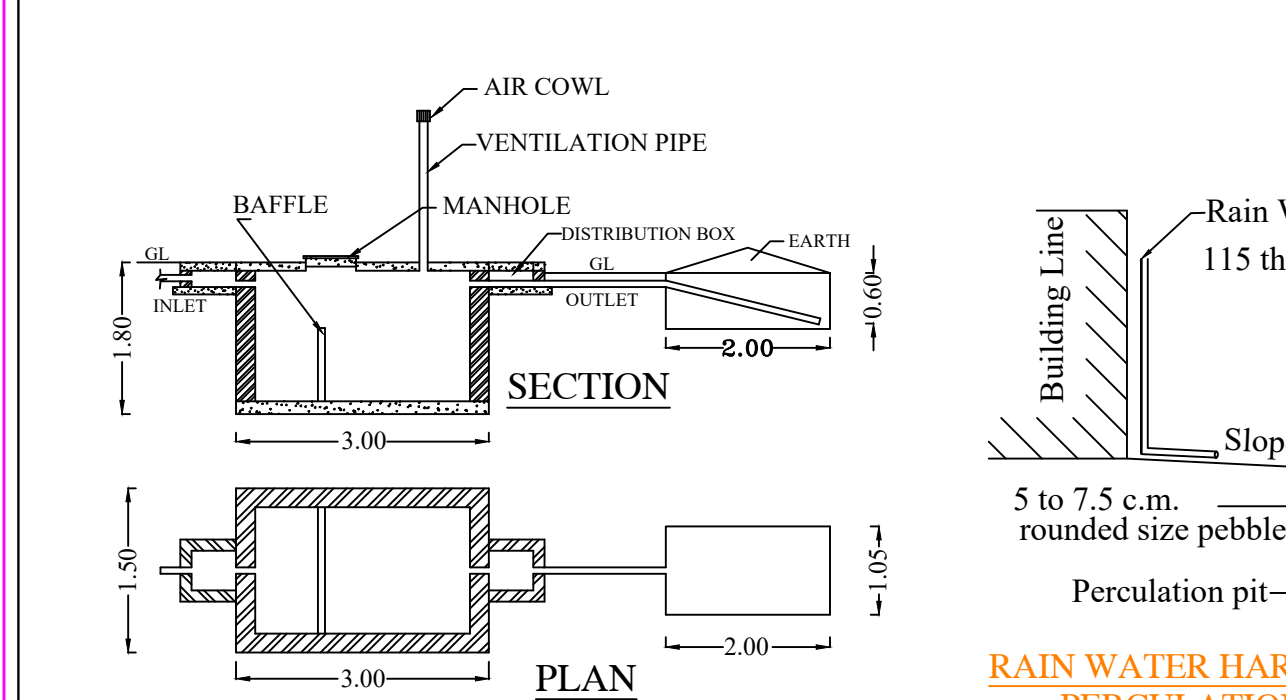
SEPTIC TANK DISPERSION TRENCH RAIN WATER HARVESTING PERCOLATION PIT
