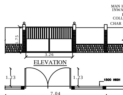
PLAN Compound wall Detail
