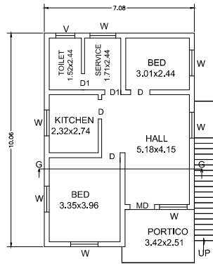
GROUND FLOOR PLAN (EXG)
