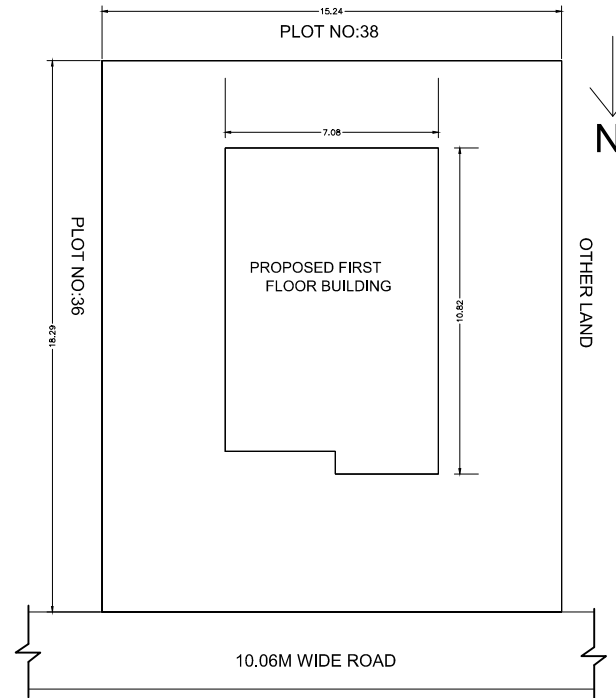
SITE PLAN
