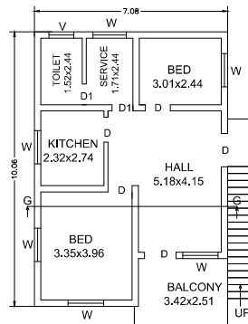
FIRST FLOOR PLAN (PRO)
