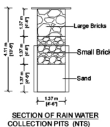
SECTION OF RAIN WATER COLLECTION PITS (NTS)
