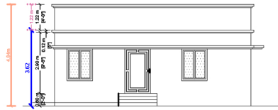
FRONT ELEVATION
