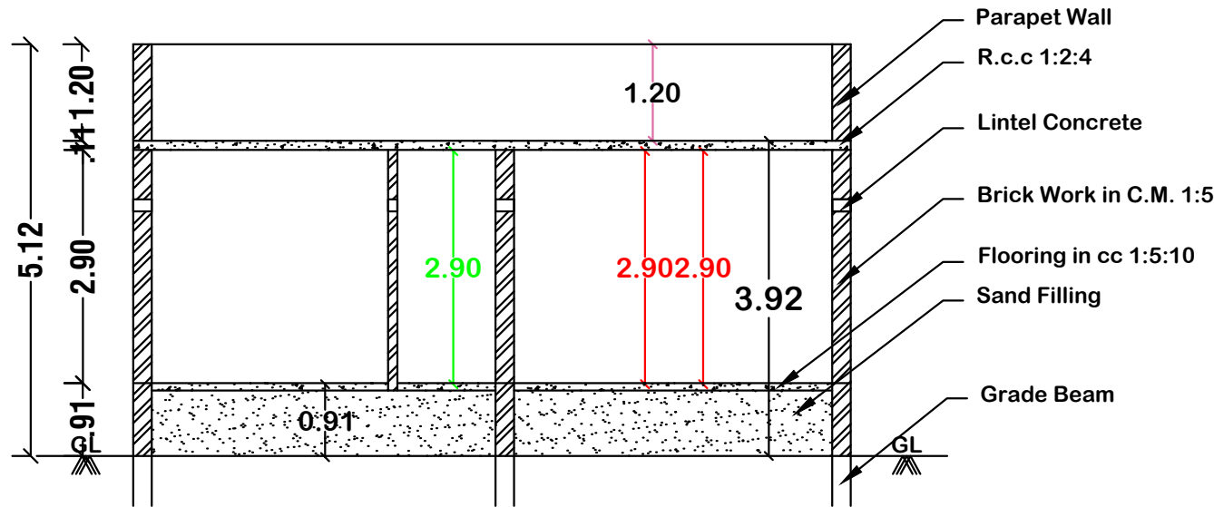
SECTION-AA
