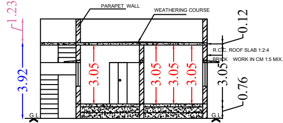
Section on-AA'
