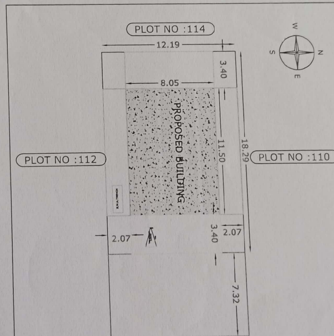
SITE PLAN
